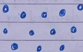
Low entropy
