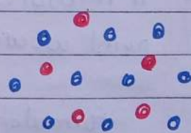
High Entropy
